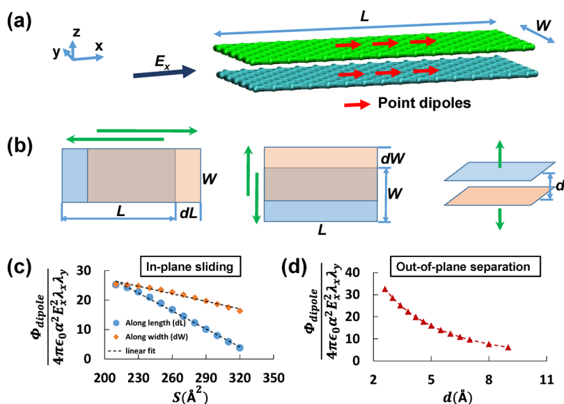
Figure 3. (a) Under an external electric field parallel to the plane of a graphene bilayer, point dipoles of the same direction as the electric field form in the graphene bilayer. (b) Schematics of in-plane sliding (left and middle panels) and out-of-plane separation (right panel) of the graphene bilayer. (c) As the two graphene layers slide off each other in the plane, the normalized dipole–dipole interaction energy decreases as the total surface area of the bilayer (e.g., 2(L + dL)W or 2L(W + dW) ) increases. (d) Similarly, as the two graphene layers separate out-of-plane, such an energy also decreases as the separation distance increases.
